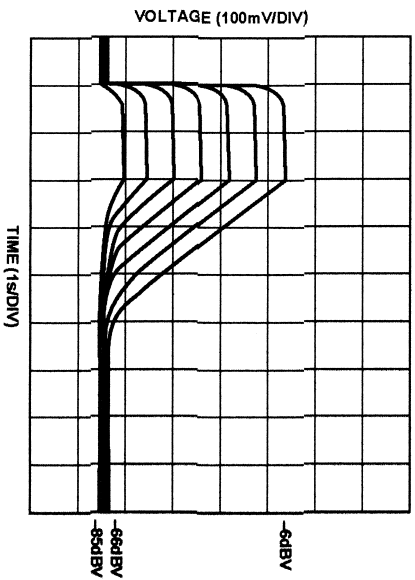
Figure 13. RMS Level Detector Performance with C_{avg} = 22 \mu F
